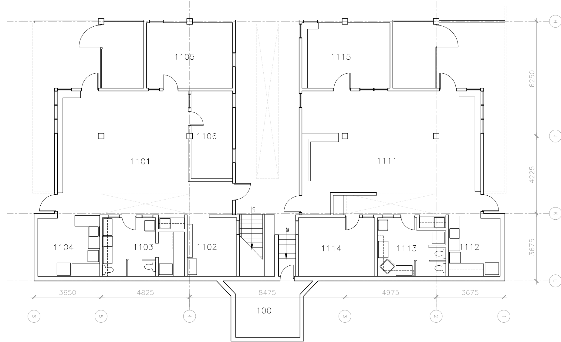
LOWER FLOOR PLAN
